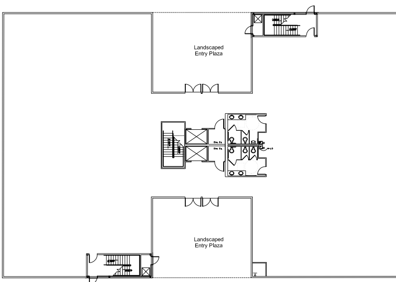
Medical Office 1st Floor 13000SF
